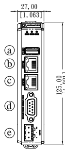
Front View
